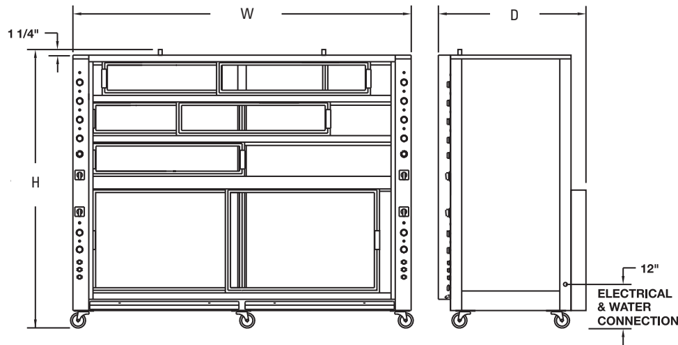
DO-PB-12-G Oven/Proofer
